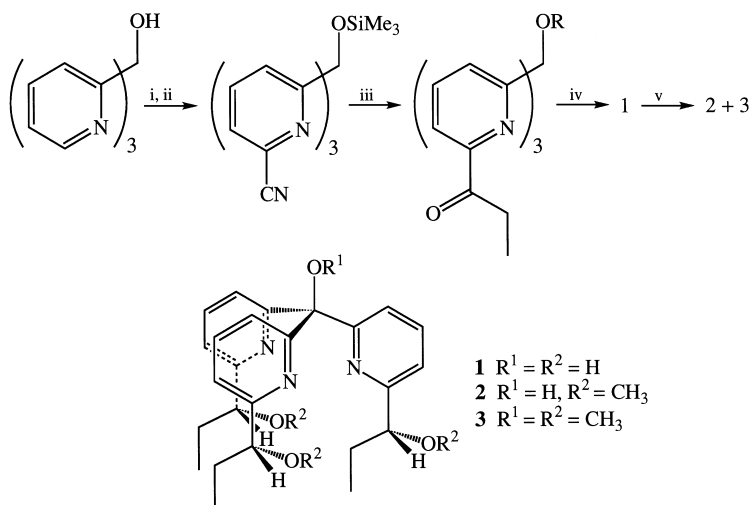
Fig. 6. The synthesis of the first chiral C_3 symmetric tris(2-pyridyl) tripod ligand, adapted from Adolfsen et al. [21] (i = m -chloroperbenzoic acid, ii = N,N -dimethylcarbamoyl chloride, trimethylsilyl cyanide, iii = EtMgBr, iv = (-)-Ipc 2 BCl, 2,2'-iminodiethanol, and v = NaH, MeI).
