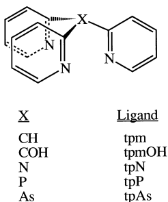
Fig. 1. Tris(2-pyridyl) tripod ligands.
