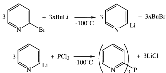
Fig. 3. Preparation of tpP as described by Keene et al. [12].
