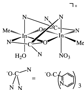
Fig. 12. The structure of [(InMe)_2\{tpmO\}_2(NO_3)(H_2O)]^+ , the first complex containing a bridging tris(2-pyridyl) tripod ligand, adapted from a general scheme from Canty et al. [62]. The tpmO-ligand is drawn without detail to aid in displaying the geometries of the iridium centers.
