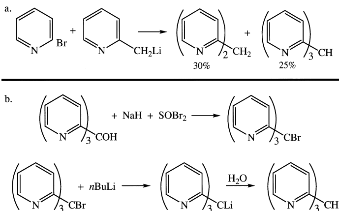
Fig. 5. Synthesis of tpm: (a) as first described by Osuch and Levine [17]; and (b) the modified synthesis as described by White and Faller [18].
