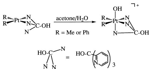
Fig. 9. Oxidation of the square planar [PtR 2 (tpmOH)] complex by water to form the octahedral [PtR 2 (tpmOH)(OH)] + complex (R = Me or Ph), adapted from Canty et al. [48]. The tpmOH ligand is drawn without detail to aid in displaying the geometries of the platinum centers.
